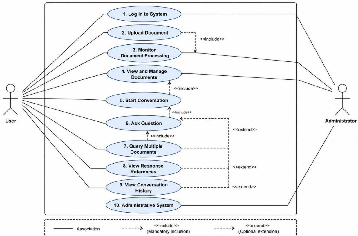
Figure 1: Use Case Diagram for the AI-powered Document Retrieval System
